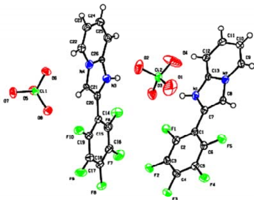
Figure 8. ORTEP view of the compound 4.
