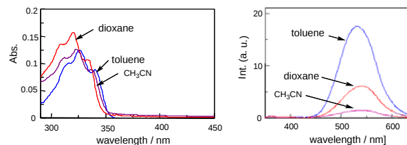
Figure 1. Absorption and fluorescence spectra of 1 in toluene, in dioxane, and in acetonitrile. [ 1 ] = 1.0 \times 10^{-5} M, \lambda_{\text{ex}} = 326 nm.
