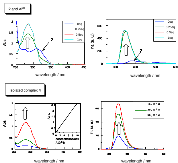
Figure 6. 2 and Al^{3+} ; Spectral change of 2 with increase of Al^{3+} . [2] = 1.0 \times 10^{-4} M, Al^{3+} : Al(ClO_4)_3 \cdot 9H_2O , solvent: acetonitrile. Isolated complex 4 ; Concentration dependence on spectra of isolated complex.
