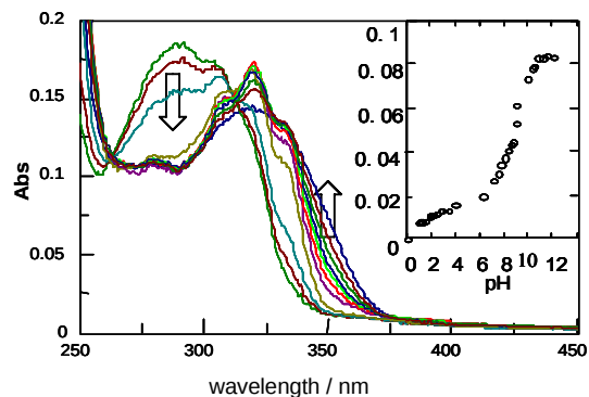
Figure 2. Spectral change of 1 between pH 1 and pH 12. [ 1 ] = 1.0 \times 10^{-5} M, solvent: MeOH / H 2 O = 9 / 1, [NaCl] = 0.1 M. The inset shows the absorbance change at 350 nm.
