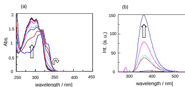
Figure 5. Absorption (a) and fluorescence (b) spectral changes with increase of Al^{3+} . [1] = 1.0 \times 10^{-4} M for absorption spectra and 1.0 \times 10^{-5} M for fluorescence spectra, [Al^{3+}] = 0-10 equivalent of 1 for absorption spectra and 0-2 equivalent of 1 for fluorescence spectra, Al^{3+} : Al(ClO_4)_3 \cdot 9H_2O , solvent: acetonitrile, \lambda_{ex} = 284 nm.
