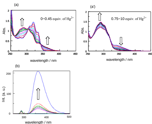
Figure 4. Absorption (a and a') and fluorescence (b) spectral changes with increase of Hg^{2+} . [1] = 1.0 \times 10^{-4} M for absorption spectra and 1.0 \times 10^{-5} M for fluorescence spectra, [Hg^{2+}] = 0-0.45 (a), 0.75-10 (a'), and 0-10 (b) equivalent of 1 , Hg^{2+} : Hg(ClO_4)_2 \cdot 3H_2O , solvent: acetonitrile, \lambda_{ex} = 284 nm.
