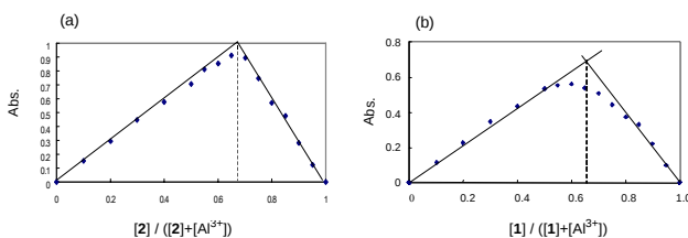
Figure 7. Job plots of (a) 2 and Al^{3+} ; (b) 1 and Al^{3+} . [2] = [1] = 1.0 \times 10^{-4} M, Al^{3+} : Al(ClO_4)_3 \cdot 9H_2O , solvent: acetonitrile.
