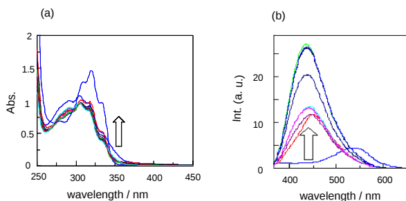
Figure 3. Absorption (a) and fluorescence (b) spectral changes with increase of Zn^{2+} . [1] = 1.0 \times 10^{-4} M for absorption spectra and 1.0 \times 10^{-5} M for fluorescence spectra, [Zn^{2+}] = 0-10 equivalent of 1 , Zn^{2+} : Zn(ClO_4)_2 \cdot 6H_2O , solvent: acetonitrile, \lambda_{ex} = 350 nm.
